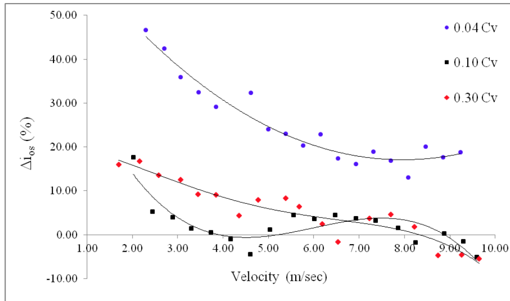
Figure 5. Percentage change in pressure gradient for 0.04 CV 0.10 CV and 0.30 CV
