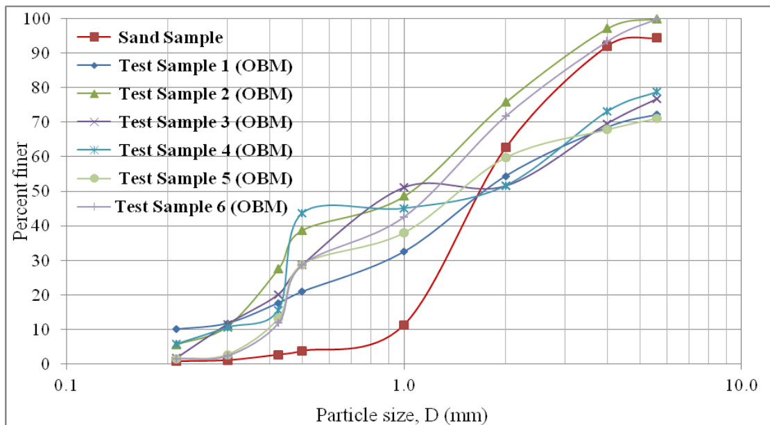
Figure 2. Particle size distribution used in the present study
