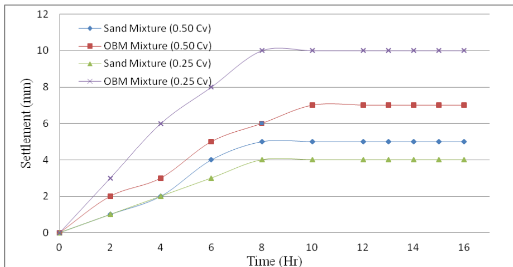
Figure 6. Settlement behavior of OBM and sand samples
