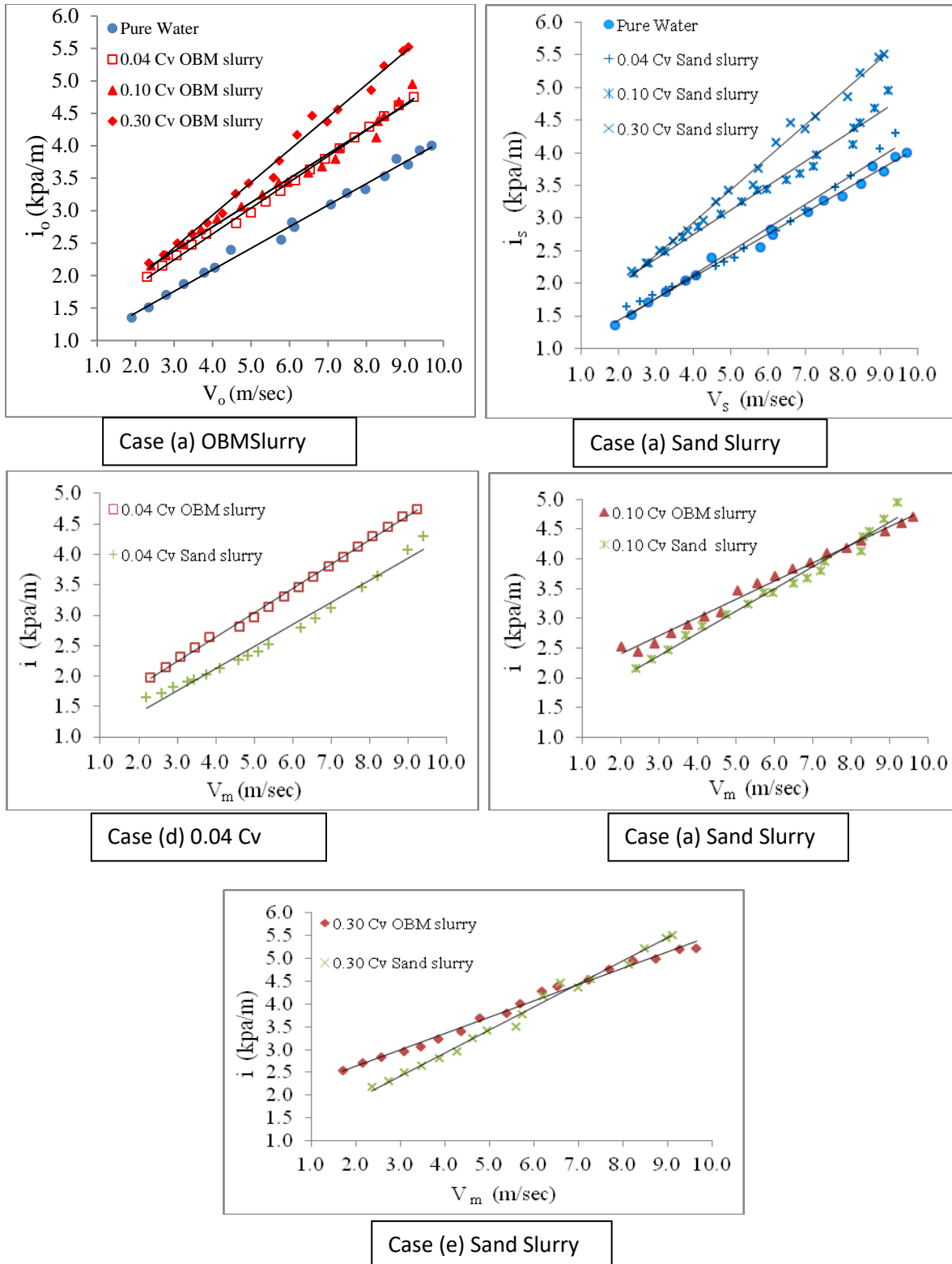
Figure 3. Pressure gradient variations with velocity for 0.04 CV, 0.10 CV and 0.30 CV for OBM and sand slurries; (case - a, b, c, d and e)
